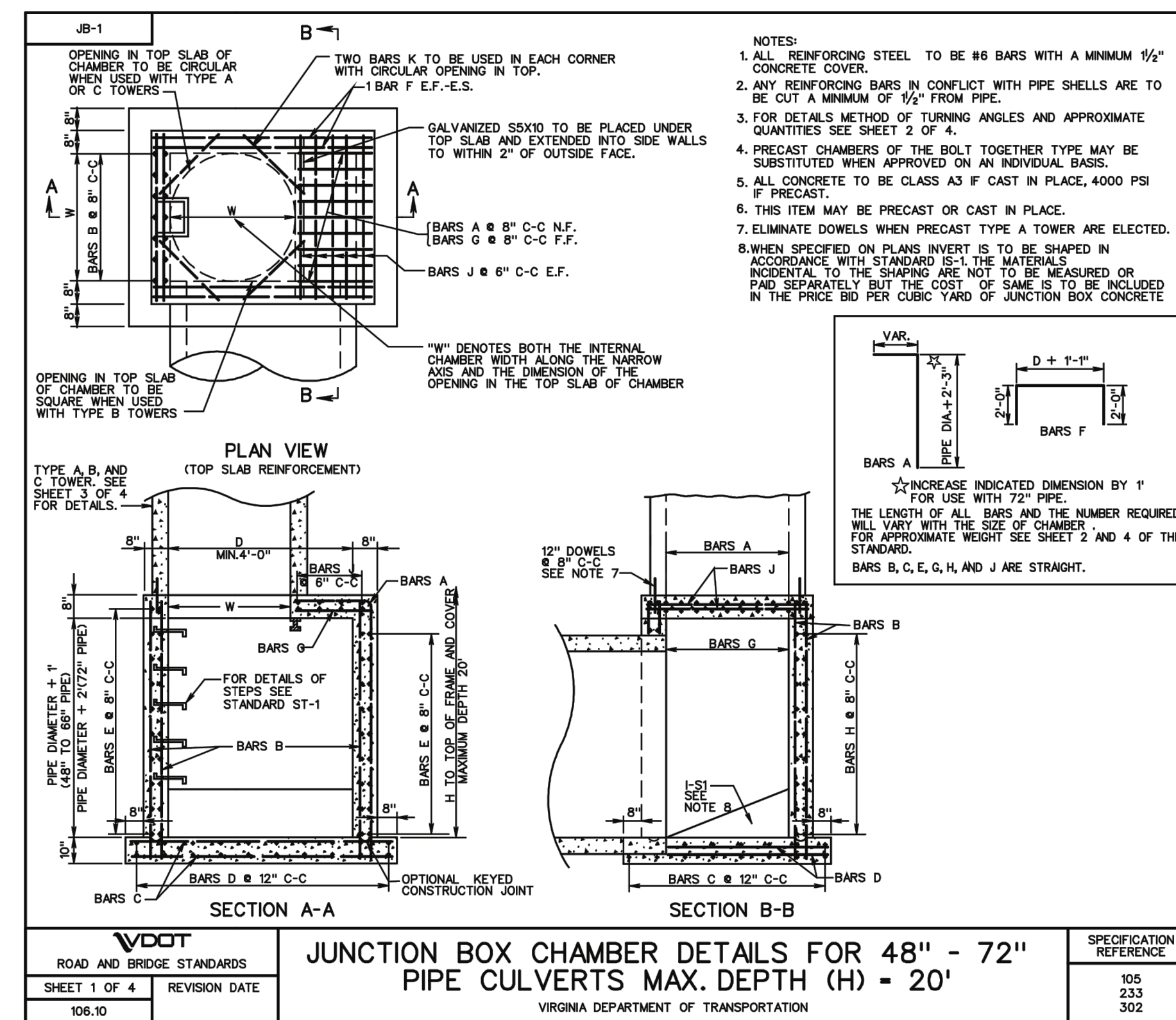
STANDARD VDOT JB-1 DETAILS
