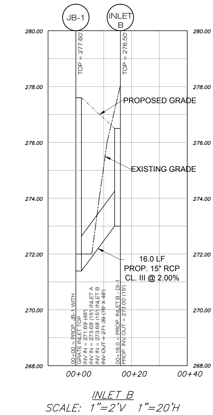
PROPOSED DI-1 INLET PROFILES
